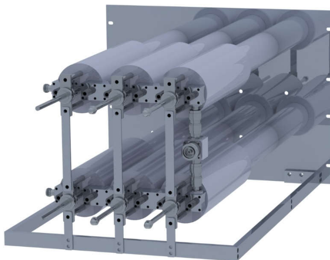
Optional 8RU Rack Mounting Kit Shown
